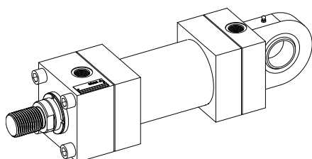
S (ISO MP5) = fixed eye with spherical bearing mounting
