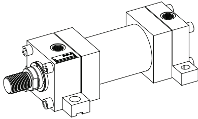
E (ISO MS2) = side feet mounting
